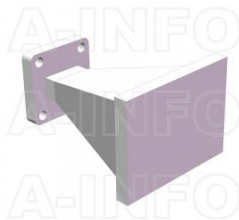
LB-42-15-ASPO Standard Gain Horn Antenna 18-26.5GHz 15dB Gain Rectangular Waveguide Interface
